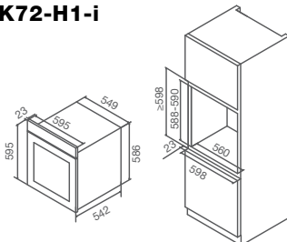
COMBI OVEN HZK72-H1-i
