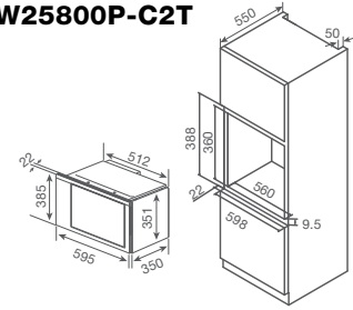
MICROWAVE OVEN HW25800K-03G HW25800P-C2T
