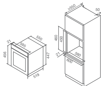
COMBI OVEN HZK46-TS3
