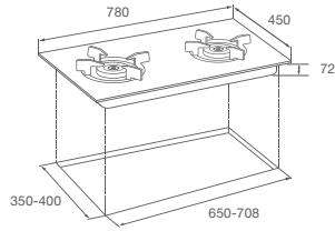
HOB GHG78215 GHG78221-i
